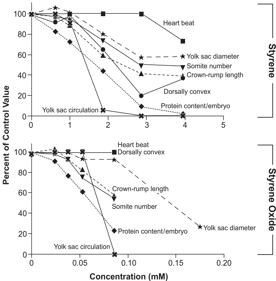
Figure 3. Concentration–response relationship of styrene and styrene oxide in rat whole embryo culture
