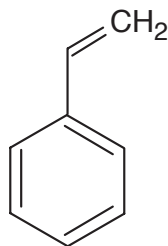
Figure 1: Chemical Structure of Styrene
