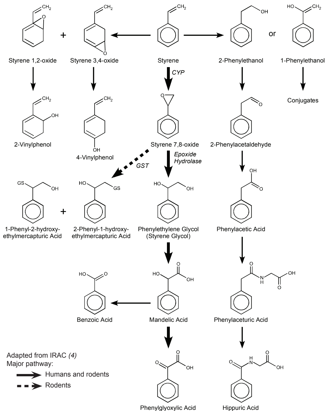
Figure 2. Metabolism of Styrene in Humans and Rodents
