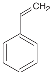
Figure 1. Chemical structure of styrene
